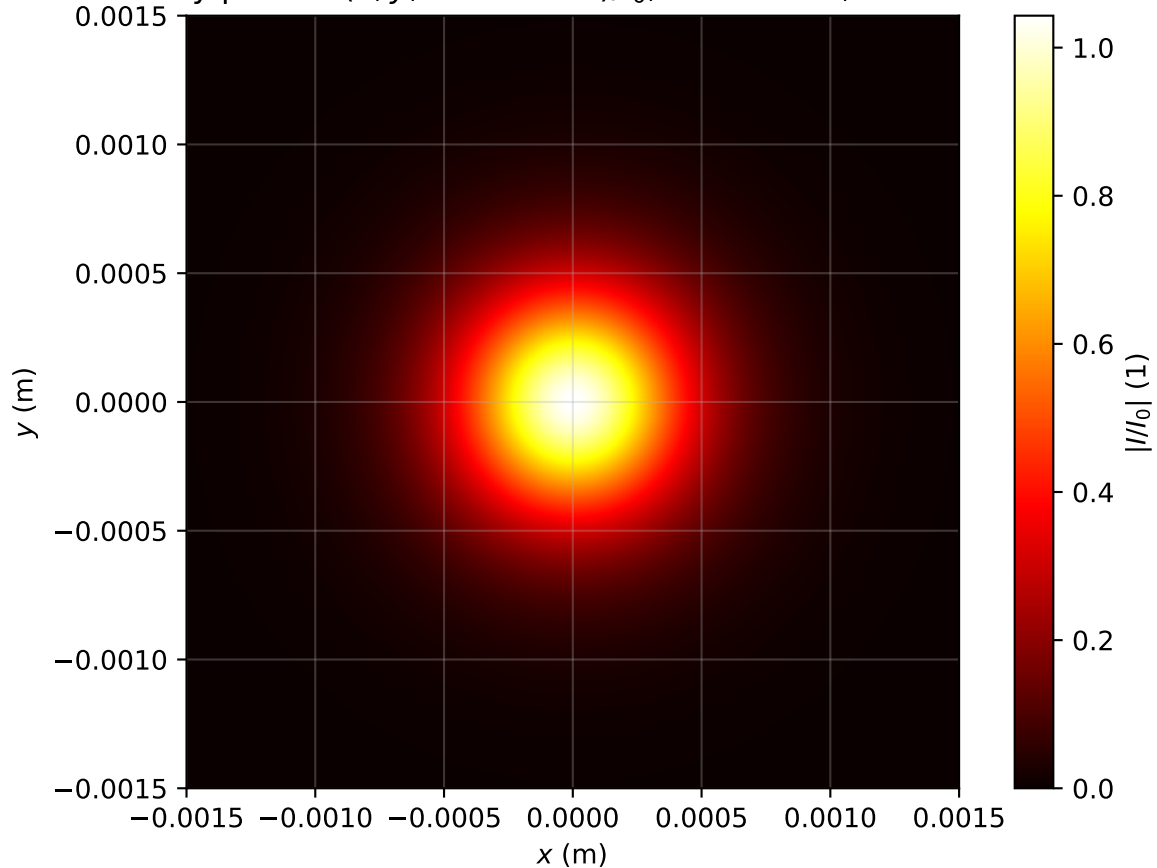
Intensity profile I(x, y, z = 2.229m)/I_0 , Pin=0.7Pcr, artificial time
